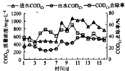
图8 工艺1 SBR对 COD_{Cr} 去除效果曲线 Fig. 8 COD_{Cr} removal efficiency of SBR at stage one
