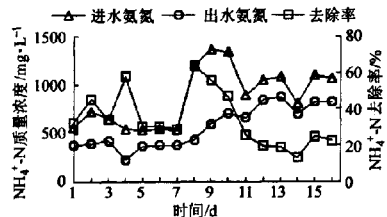
图9 工艺1 SBR对 NH_4^+-N 去除效果曲线 Fig. 9 NH_4^+-N removal efficiency of SBR at stage one
